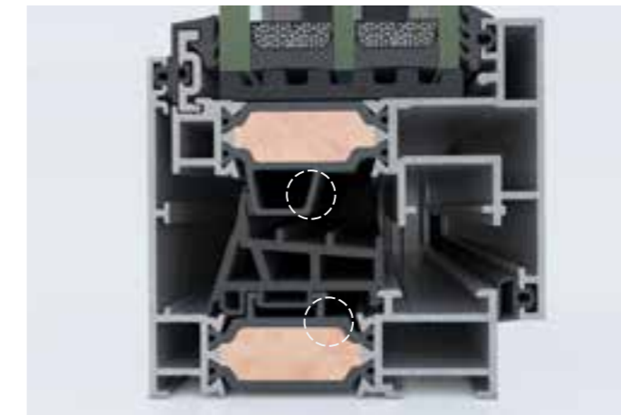
WIDE INSULATING BARS 32mm Wide insulating bars of 32mm with glass fiber re-enforcement 25%, are applied to all system profiles, offering high thermal insulation levels and extra rigidity.
