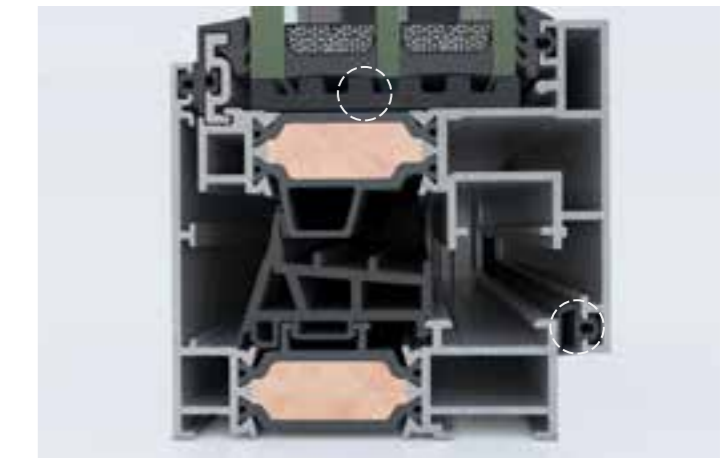
CO-EXTRUDED GASKET & FOAM INSULATING PROFILE Co-extruded gasket is used in the perimetrical area of the window, improving energy performance. Whilst foam insulating profile is fitted below the glazing zone, minimizing thermal energy loss.
